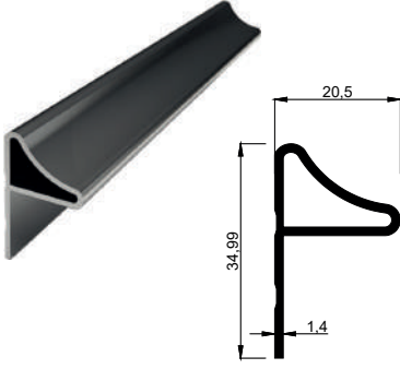
KALIP NO 4117 Kg / m: 0,584
